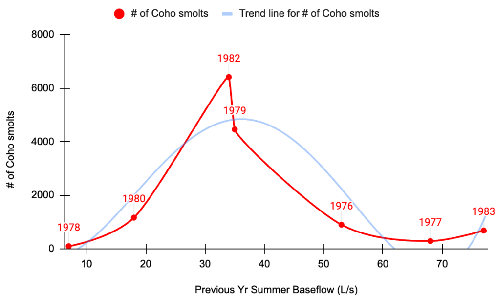
Figure 1. Smolt counts from 1976-1983 plotted against previous summer baseflows.
