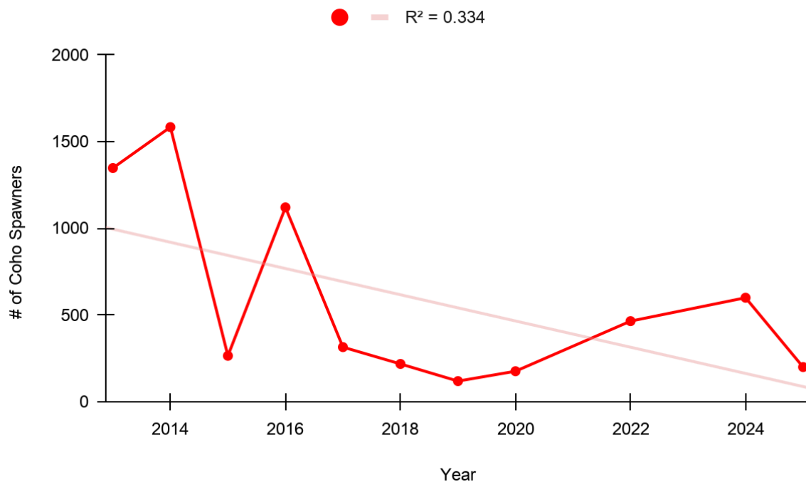
Figure 11. Linear trend of Coho spawner return counts from 2013-2025.
