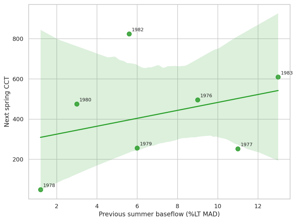
Figure 2. Relationship between CCT counts and previous summer baseflow presented as %LTMAD.
